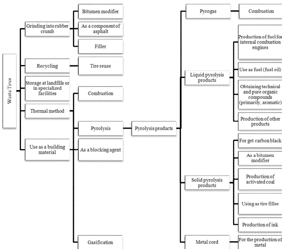
Fig. 2. Methods of WAT disposal and their general areas of application
