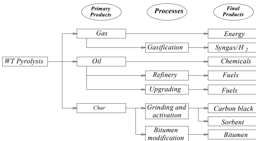
Fig. 3. Products obtained as a result of WAT pyrolysis and their areas of application
