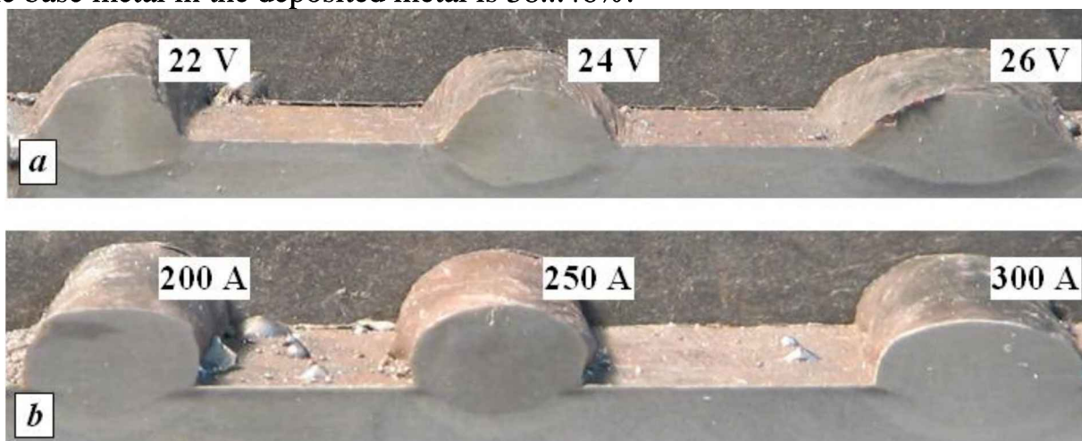
Figure 1. Macro-grinding of rollers deposited with powder-coated wire PP-Np-150Kh5T4M Ø 1.8 mm under AN-26P flux at different voltages at the same current of 250 A (a) and on different currents at the same voltage of 24 V (b)
